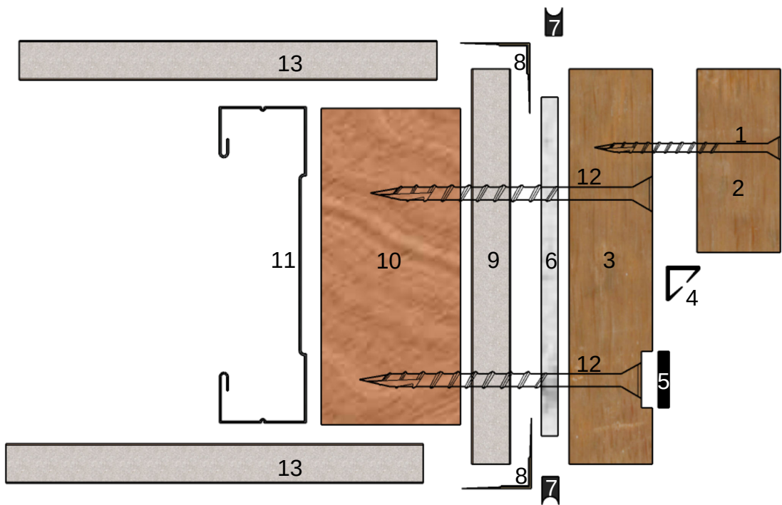
Exploded Make-up 2D
