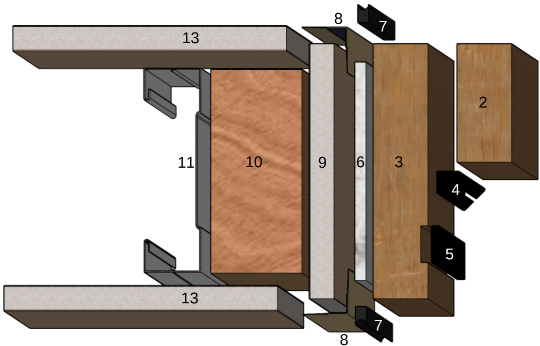
Exploded Make-up 3D
