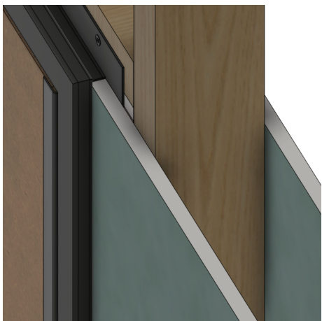
Align Noiseline Gib With Top GIB Groove
